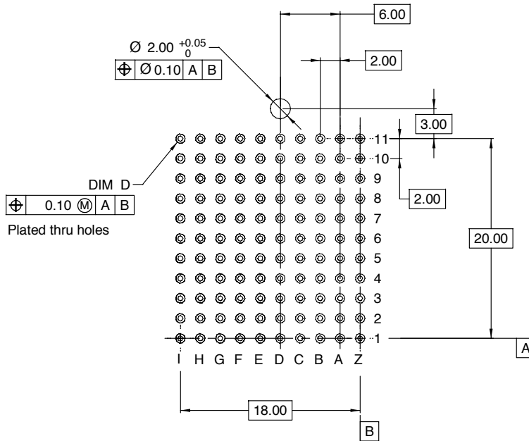
Recommended PCB hole mounting pattern
